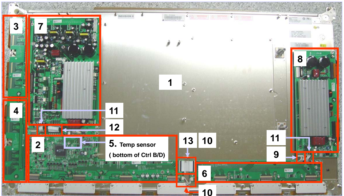
Fig B、 Model name labeling part、 Part arrangement plan (Panel back)
