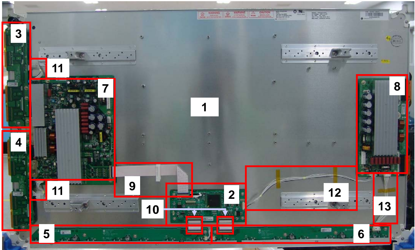
Fig A、 Model name labeling part、 Part arrangement plan (Panel back)
